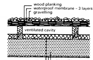
6 Cold roof - heavy construction
